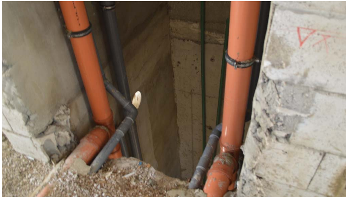
Figure 20: Drainage installations in shafts
